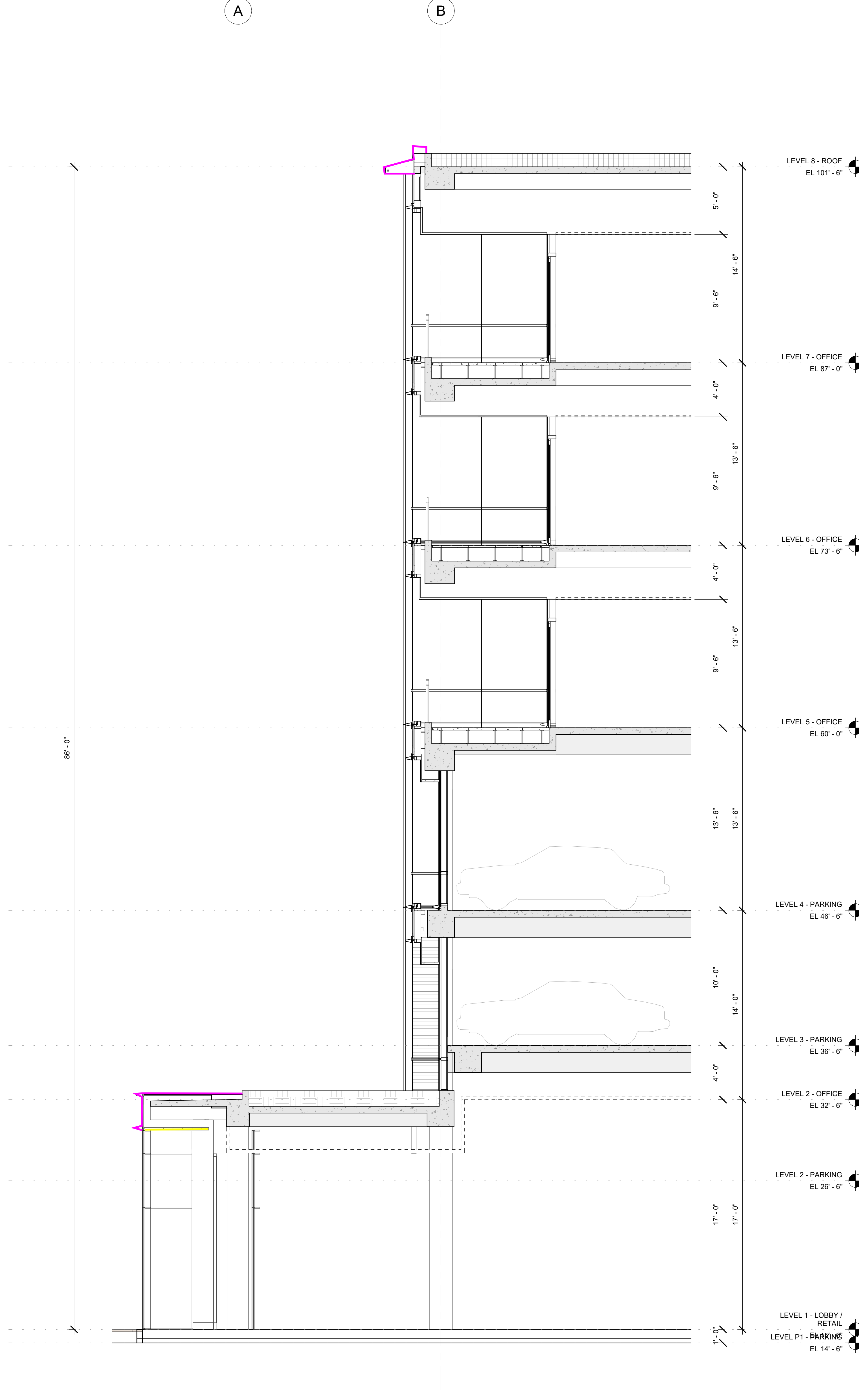
2 WALL SECTION 1/4" = 1'-0"
